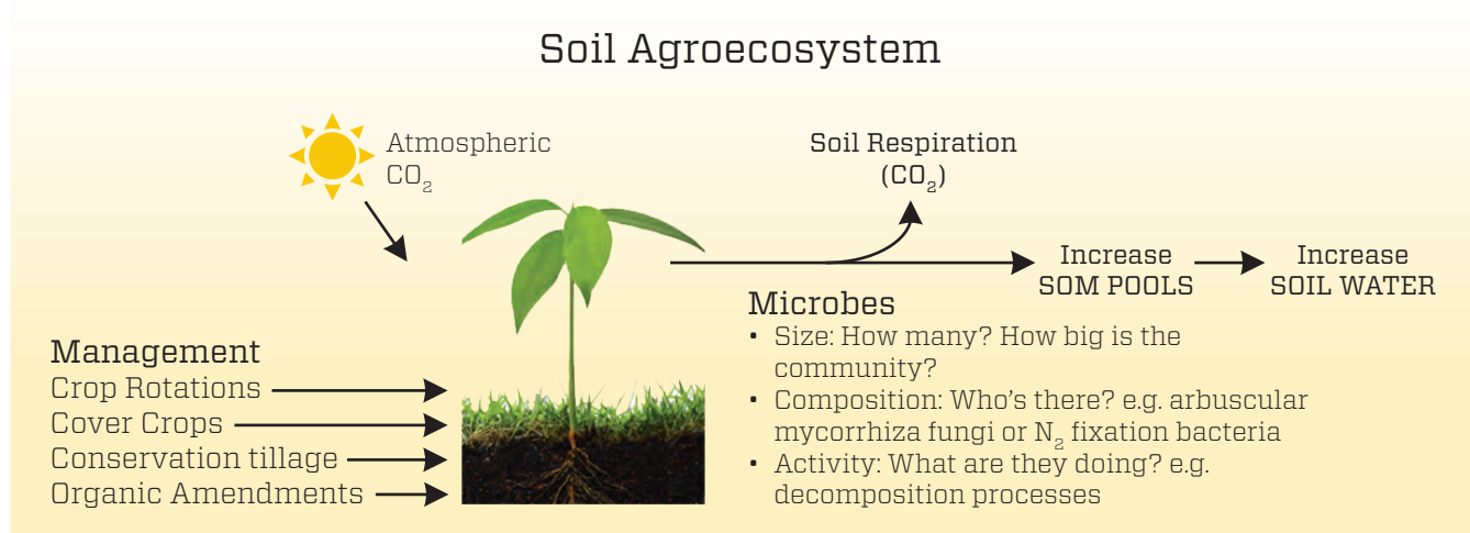
Figure 1. The coupled metabolisms of soil microorganisms during the decomposition of carbon (C) inputs builds soil organic matter (SOM) and releases carbon dioxide (CO 2 ). In agroecosystems, SOM is the manifestation of a dynamic equilibrium of C inputs and C outputs from decomposition, leaching, and soil erosion.
