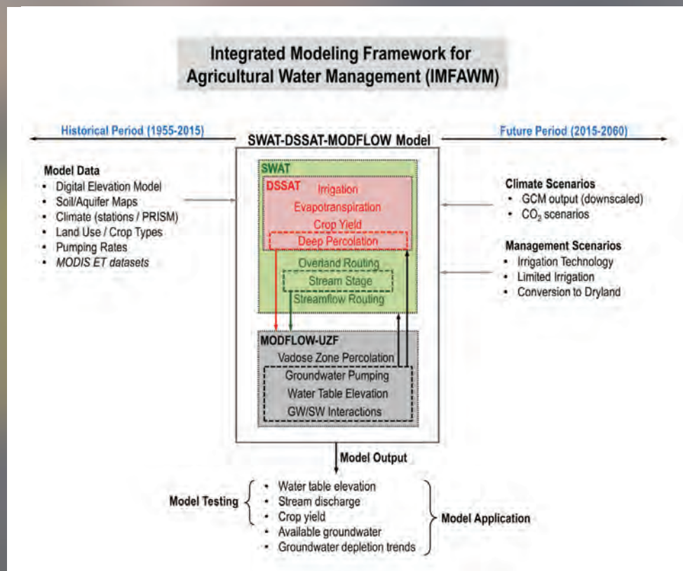
Figure 1. A schematic of an integrated modeling framework for agricultural water management in the Ogallala Aquifer Region.
